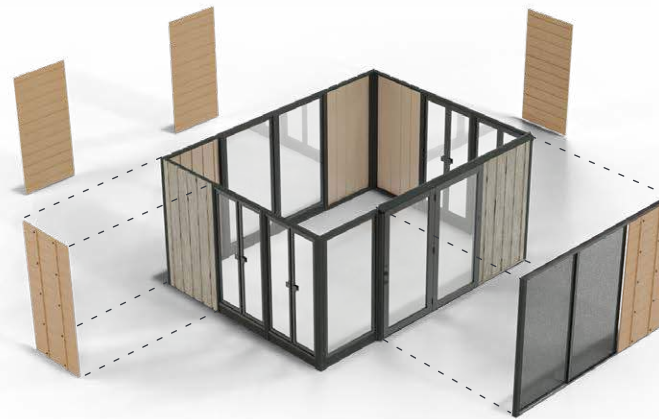
Base model with Cedar Panels and Sliding Screen Doors
