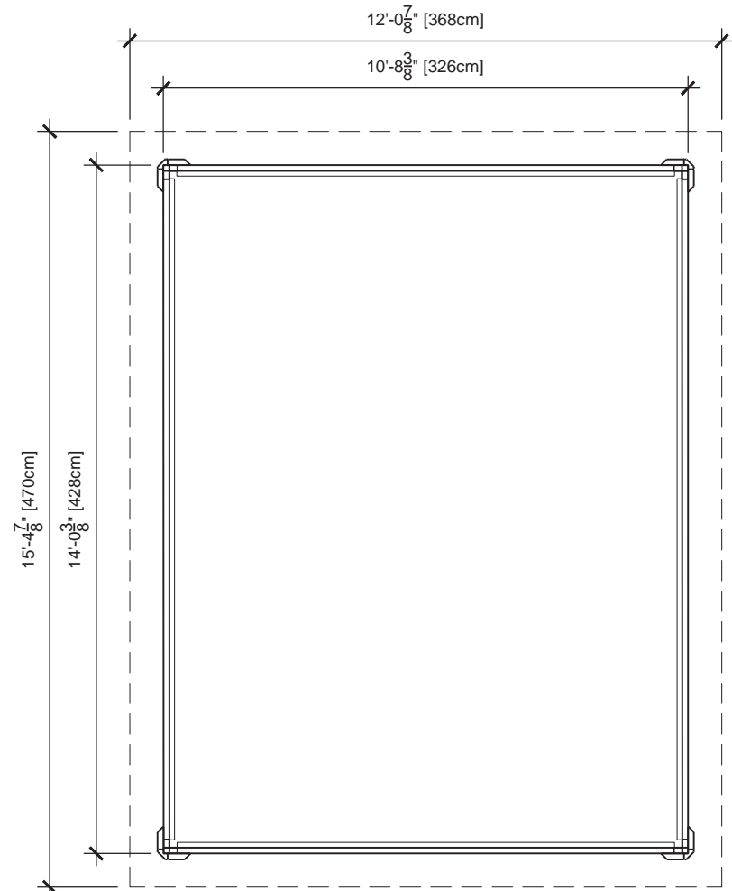
Footprint Plan
